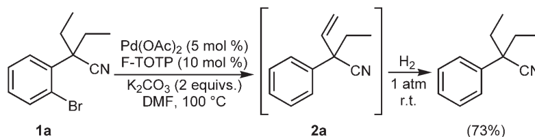
Scheme 3. C(sp^3) -H activation/hydrogenation one-pot process.
