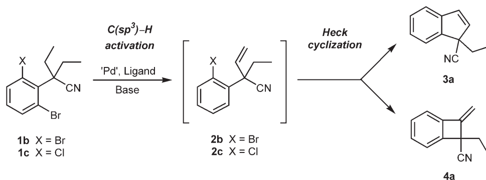
Scheme 2. C( sp^3 )-H activation/Heck cyclization cascade reaction.
